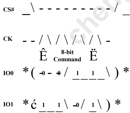
Figure 7 — Fetch SFDP (2S-2S-2S) Mode Timing Diagram
